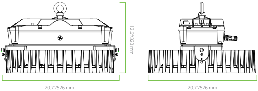
PS600W Weight: 38.50 lbs/ 17.50 kg
