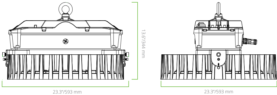
PS800W Weight: 49.30 lbs/ 22.40 kg
