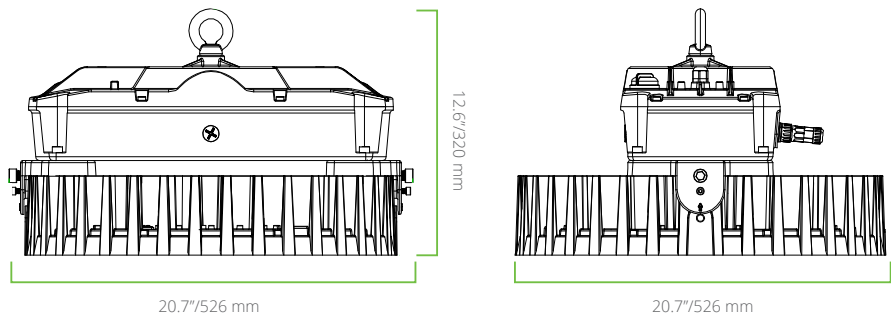
PS450W Weight: 35.90 lbs/ 16.30 kg
